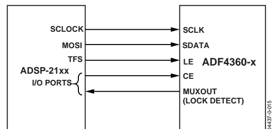
Figure 18. ADSP-21xx to ADF4360-x Interface
