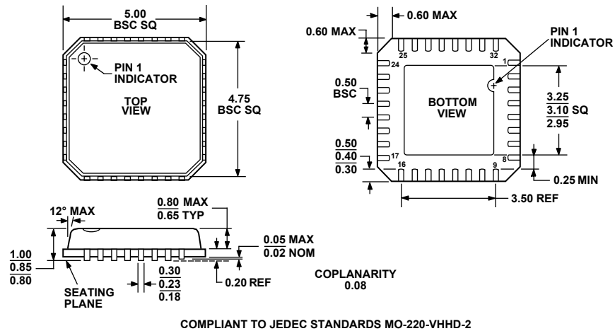
Figure 11. 32-Lead Frame Chip Scale Package [LFCSP] (CP-32)
