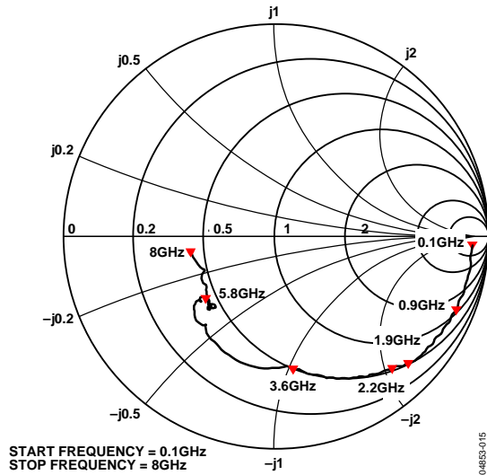
Figure 15. Input Impedance vs. Frequency; No Termination Resistor on INHI
