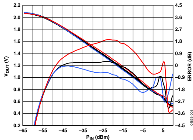
Figure 8. V_{OUT} and Log Conformance vs. Input Amplitude at 8 GHz, Typical Device
