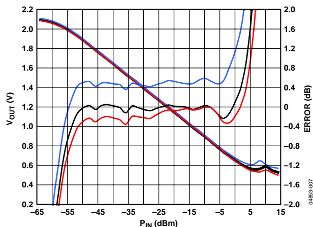
Figure 7. V_{OUT} and Log Conformance vs. Input Amplitude at 2.2 GHz, Typical Device
