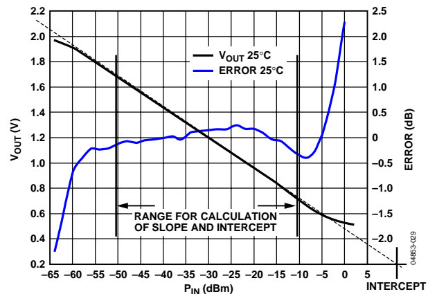
Figure 29. Typical Output Voltage vs. Input Signal
