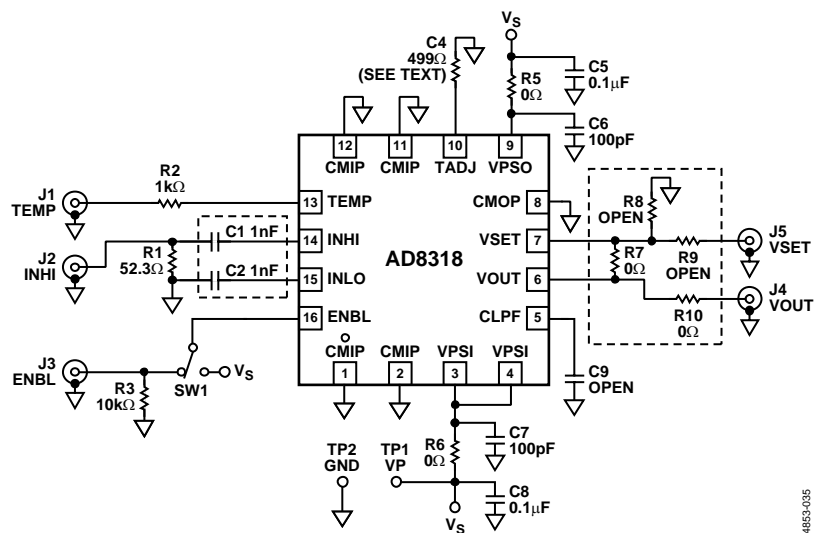
Figure 45. Evaluation Board Schematic (Rev A)
