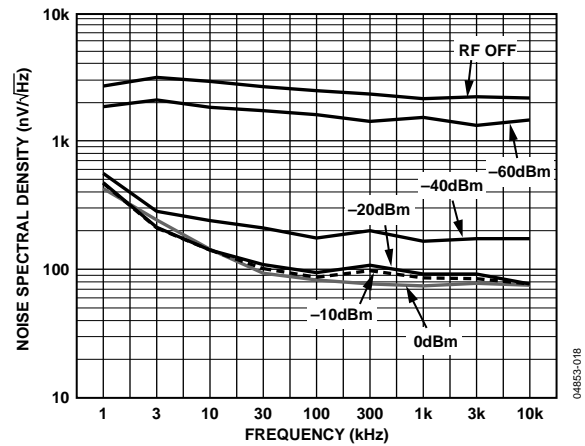
Figure 18. Noise Spectral Density of Output; C_{LPF} = Open
