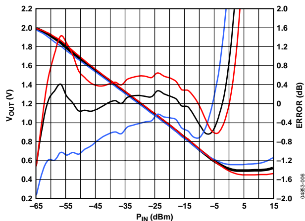
Figure 6. V_{OUT} and Log Conformance vs. Input Amplitude at 5.8 GHz, Typical Device, T_{ADJ} = 1000\ \Omega
