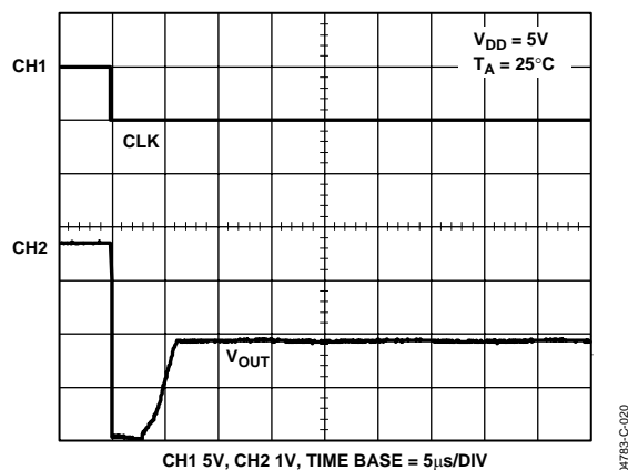
Figure 20. Exiting Power-Down
