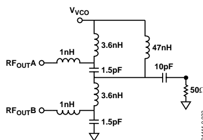
Figure 22. Balun for Combining ADF4360-1 RF Outputs
