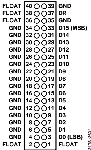
Figure 26. Single-Channel Connector Pin Diagram— Top View (HSC-ADC-EVAL-SC)
