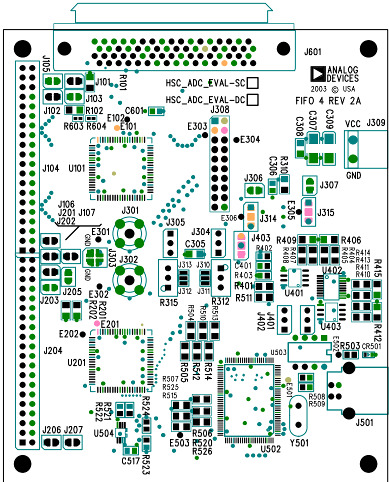
Figure 34. Assembly—Primary Side
