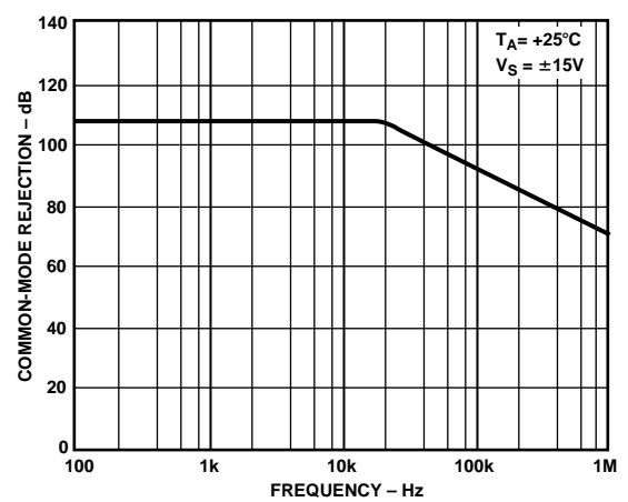
Figure 31. Common-Mode Rejection vs. Frequency @ \pm 15 V
