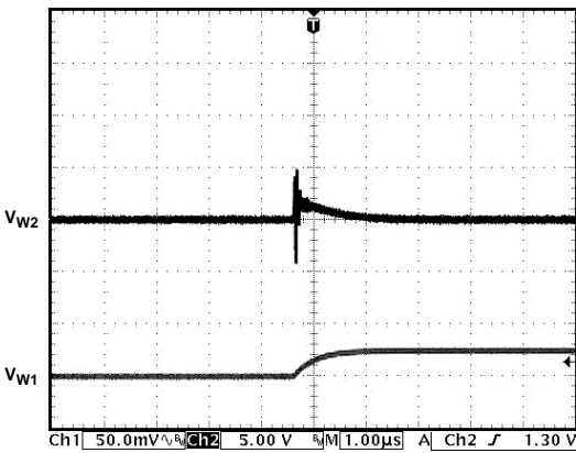
Figure 24. Analog Crosstalk
