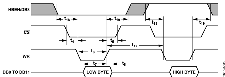
Figure 41. AD7938/AD7939 Parallel Interface—Write Cycle Timing for Byte Mode Operation ( \overline{W/\overline{B}} = 0 )
