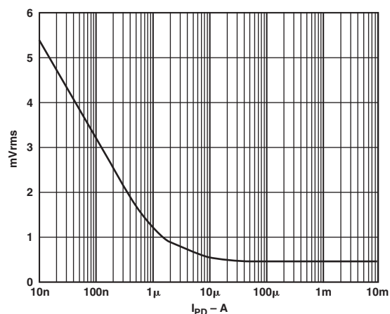
TPC 18. Total Wideband Noise Voltage at V_{OUT} vs. I_{PD} ( G = 1 )
