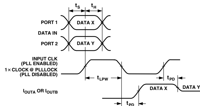
Figure 1. I/O Timing
