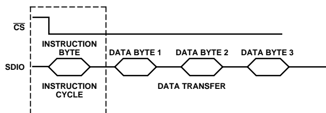
Figure 51. Using SDIO as a Read/Write Transfer
