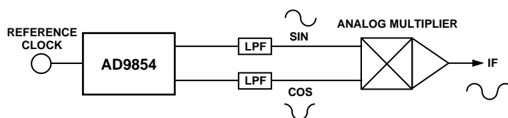
Analog Frequency Double Application
