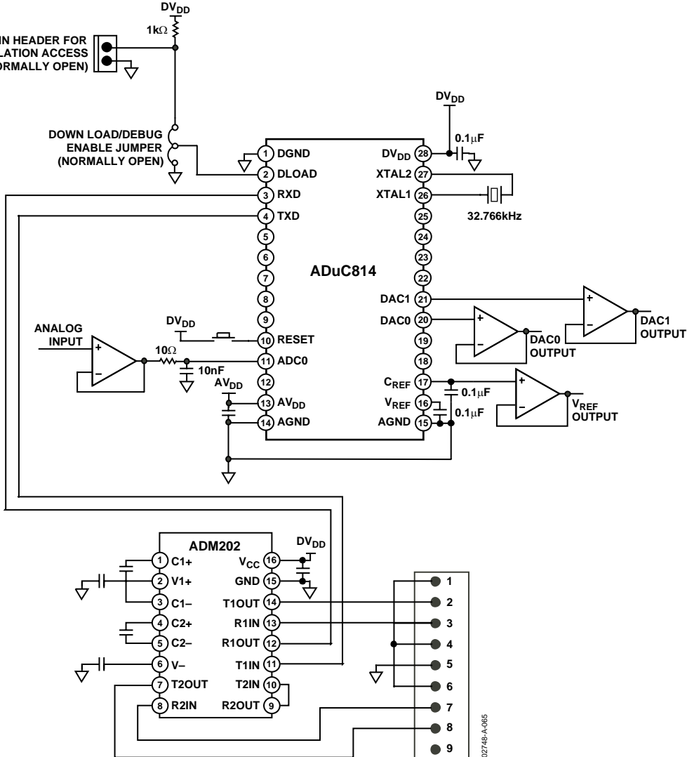
Figure 59. Typical ADuC814 System Connection Diagram
