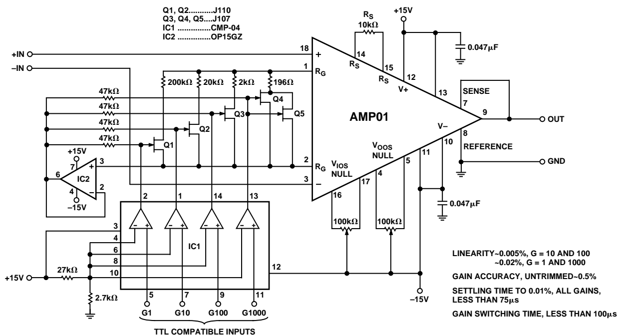
Figure 39. The AMP01 Makes an Excellent Programmable-Gain Instrumentation Amplifier. Combined Gain-Switching and Settling Time to 13 Bits Falls Below 100 \mu s . Linearity Is Better than 12 Bits over a Gain Range 1 to 1000.
