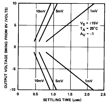
SETTLING TIME
