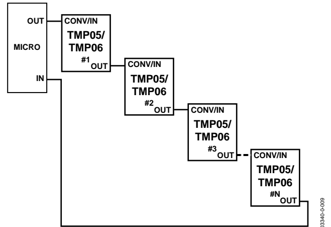
Figure 25. Daisy-Chain Structure
