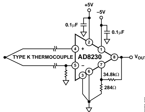
Figure 2. Thermocouple Measurement
