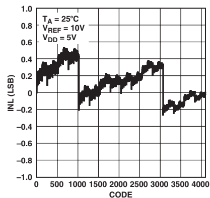
TPC 3. INL vs. Code (12-Bit DAC)
