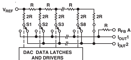
Figure 4. Simplified Ladder
