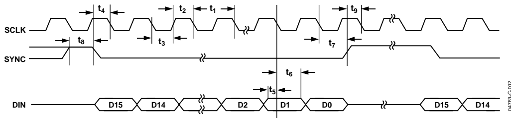
Figure 2. Timing Diagram
