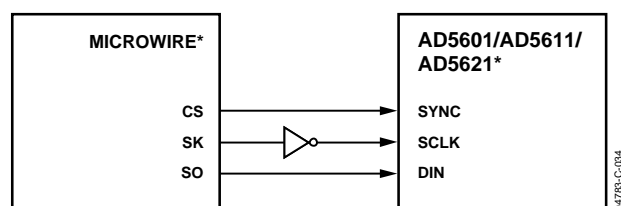
Figure 33. AD5601/AD5611/AD5621 to MICROWIRE Interface
