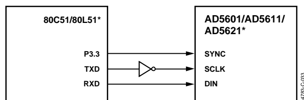
Figure 32. AD5601/AD5611/AD5621 to 80C51/80L51 Interface
