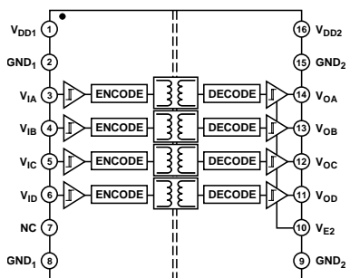
Figure 1. ADuM1400 Functional Block Diagram
