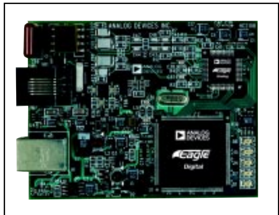
Eagle-USB reference design board shown
