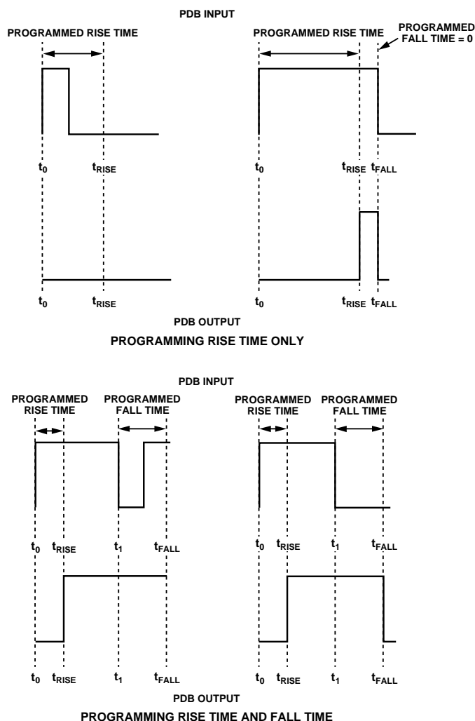
Figure 22. Programmable Delay Block (PDB) Functionality
