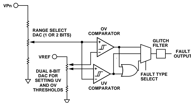
Figure 18. Positive Programmable Supply Fault Detector
