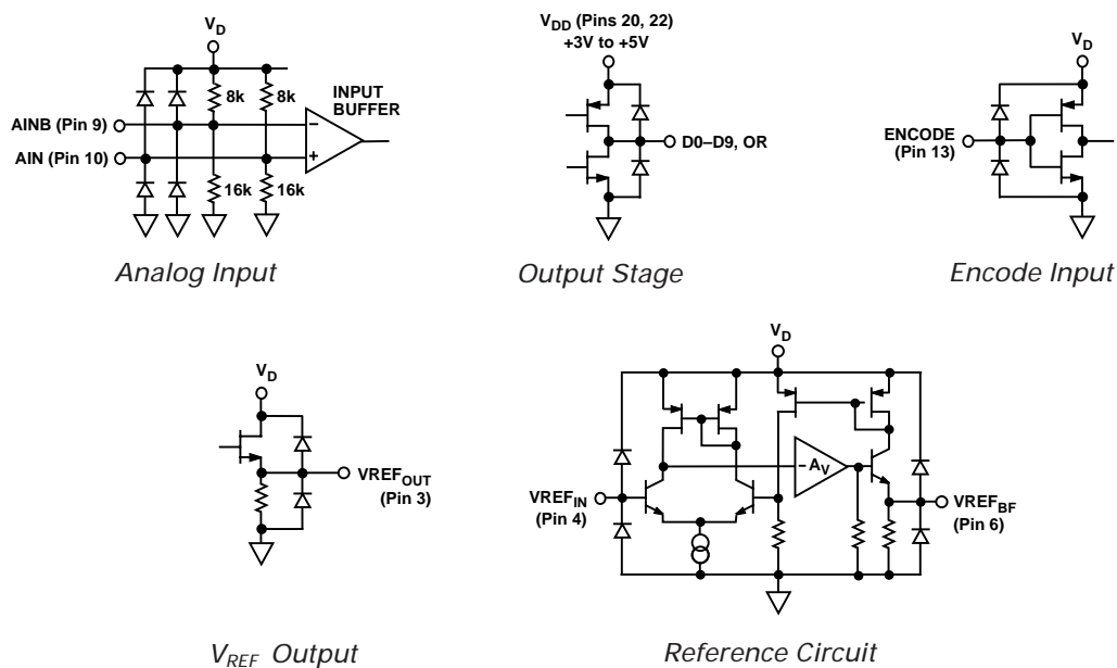
Figure 3. Equivalent Circuits
