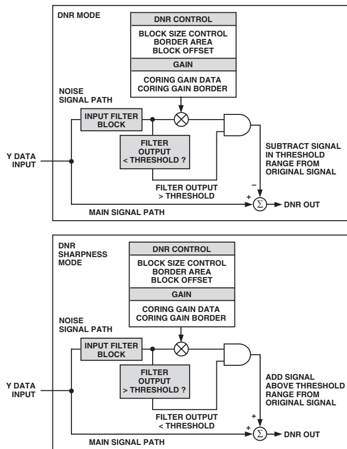
Figure 47. DNR Block Diagram
