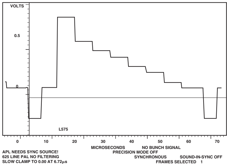
Figure 110. PAL Luma
