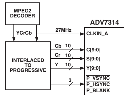
Figure 22. Progressive Scan Input Mode
