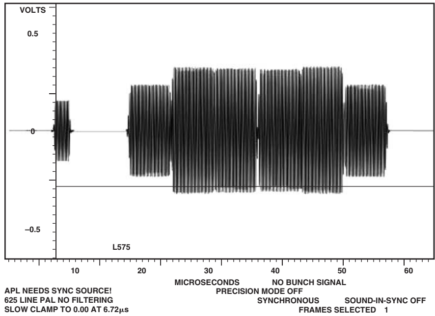
Figure 109. PAL Chroma
