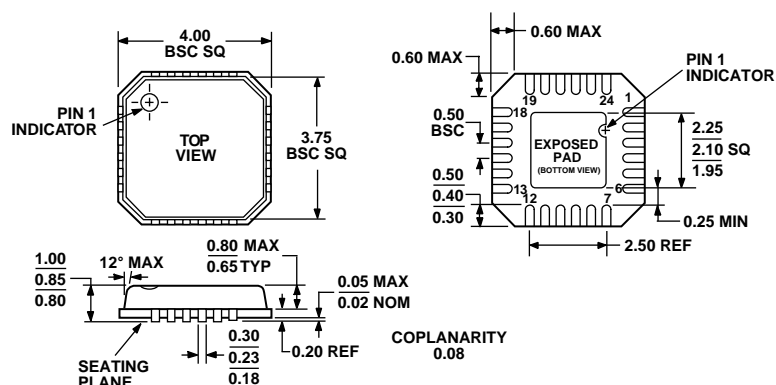
Figure 34. 24-Lead Lead Frame Chip Scale Package [LFCS]
