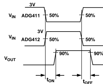
Figure 17. Switching Times
