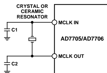
Figure 14. Crystal/Resonator Connection for the AD7705/AD7706
