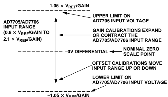
Figure 13. Span and Offset Limits
