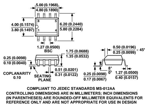
Figure 15. 8-Lead Standard Small Outline Package [SOIC] Narrow Body (R-8) Dimensions shown in millimeters and (inches)
