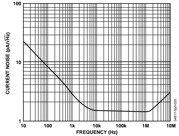
Figure 12. Input Current Noise vs. Frequency, V_S = \pm 6\text{ V}
