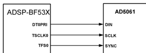
Figure 2X. AD5061 to Blackfin ADSP-BF53X Interface
