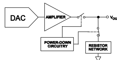
Figure 24. Output Stage During Power-Down
