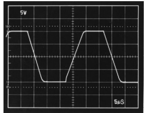
Figure 23. Unity Gain Inverter Large Signal Pulse Response
