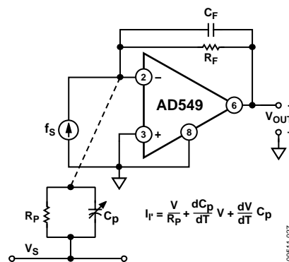
Figure 27. Sources of Parasitic Leakage Currents
