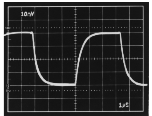
Figure 24. Unity Gain Inverter Small Signal Pulse Response
