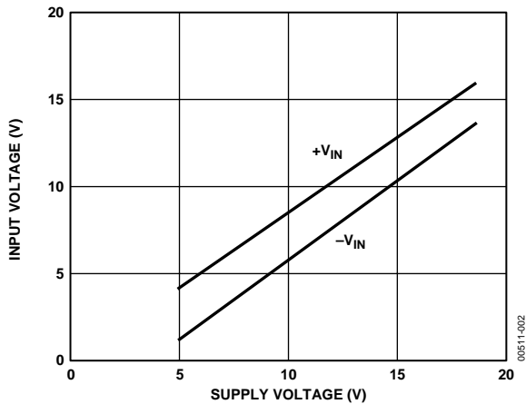
Figure 2. Input Voltage Range vs. Supply Voltage
