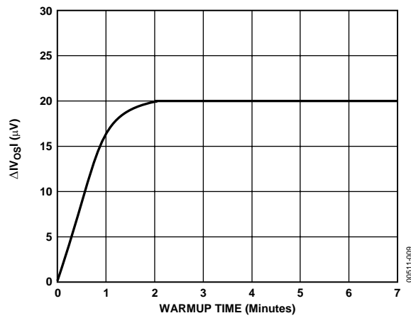
Figure 9. Change in Offset Voltage vs. Warm-Up Time
