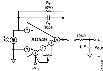
Figure 41. Photodiode Preamp
