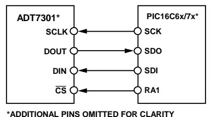
Figure 16. ADT7301 to PIC16C6x/7x Interface
