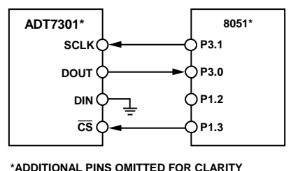
Figure 15. ADT7301 to 8051 Interface
