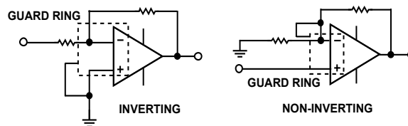
Figure 47. Guard-Ring Configurations
