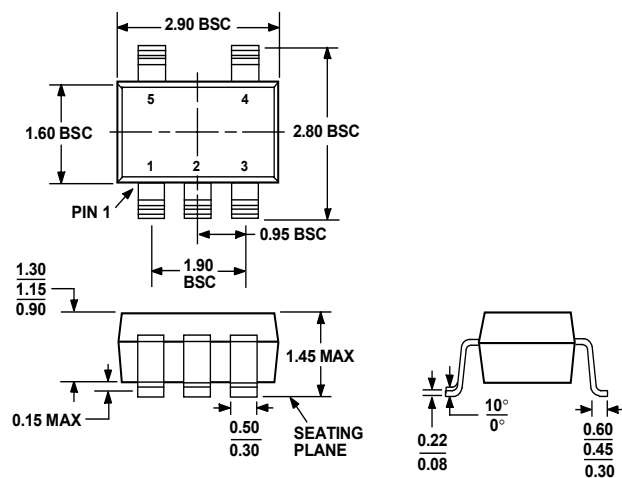
COMPLIANT TO JEDEC STANDARDS MO-178AA Figure 61. 5-Lead Plastic Surface Mount Package [SOT-23] (RT-5) Dimensions shown in millimeters
