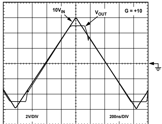
Figure 17. Output Overdrive Recovery
