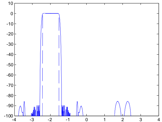
Figure 42. Interpolation/Modulation Combination of -2f_{DAC}/8 Filter in Odd Mode
