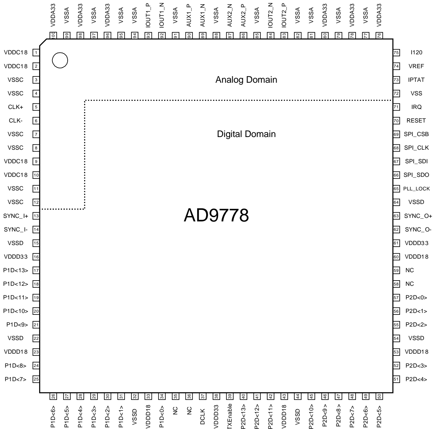
Figure 2. Pin Configuration
