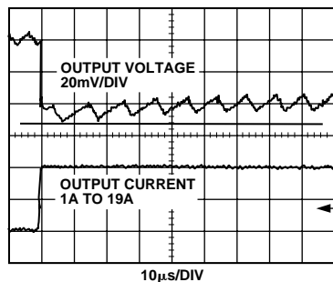
Figure 10. Transient Response, 1 A to 19 A of Figure 2 Circuit
