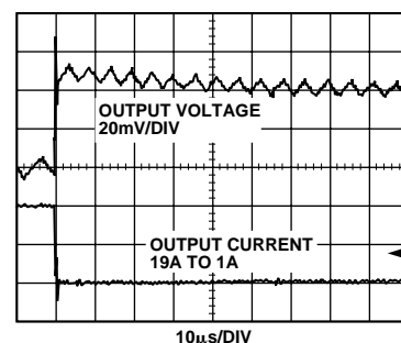
Figure 9. Transient Response, 19 A to 1 A of Figure 2 Circuit
