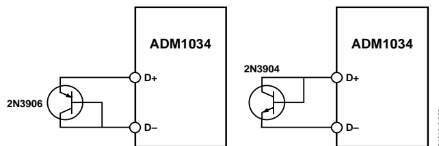
Figure 27. Measuring Temperature by Using Discrete Transistors
