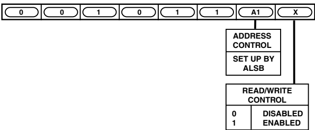
Figure 4. Slave Address
