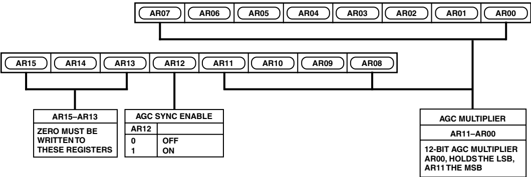
Figure 20. AGC Registers 0–1
