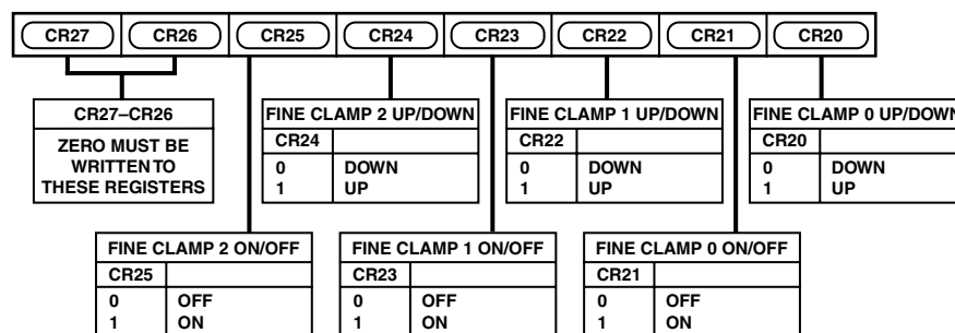
Figure 23. Clamp Register 2
