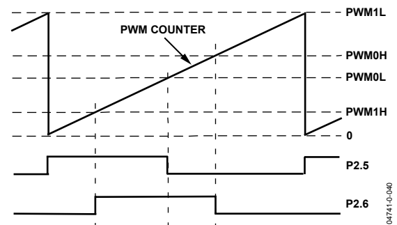
Figure 40. PWM Mode 2
