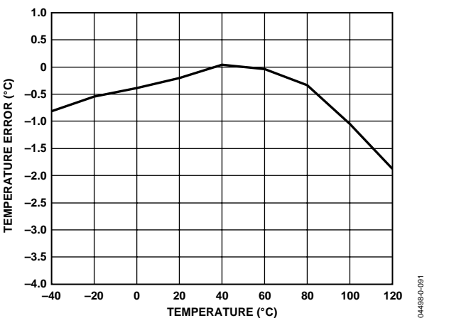
Figure 13. Internal Temperature Error vs. ADT7467 Temperature
