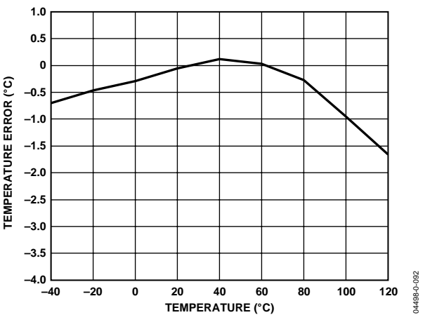
Figure 14. Remote Temperature Error vs. ADT7467 Temperature
