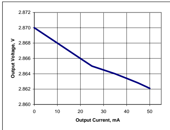
TPC3, LDO6a load regulation
