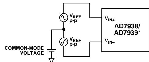
Figure 24. Differential Input Definition
