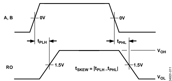
Figure 11. Receiver Propagation Delay
