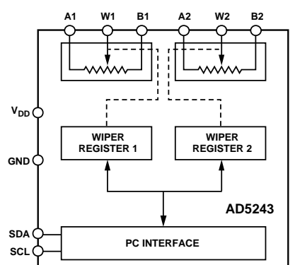
Figure 1. AD5243
