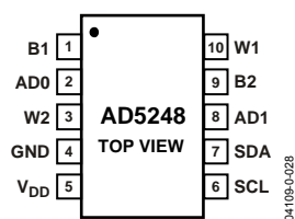
Figure 4. AD5248 Pin Configuration
