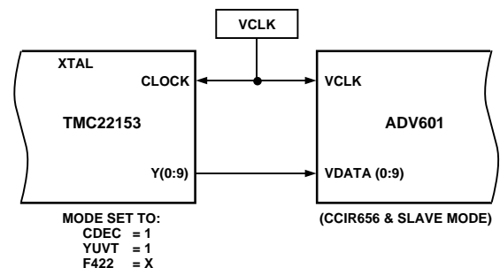
Figure 22. ADV601 and TMC22153 Example CCIR-656 Mode Interface
