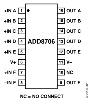
Figure 1. 16-Lead TSSOP
