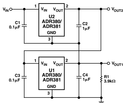
Figure 2. Stacking Voltage References with the ADR380/ADR381
