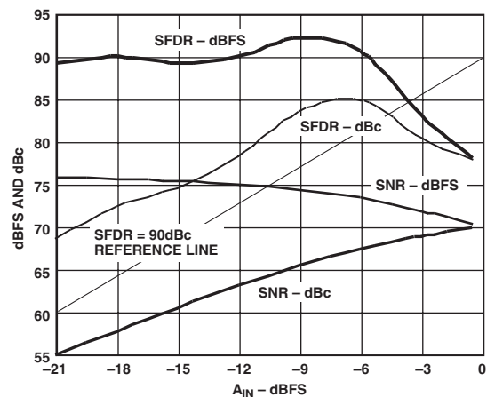
TPC 30. Driving ADC Inputs with Transformer and Balun SNR/SFDR vs. A_{IN} , f_{IN} = 190 MHz
