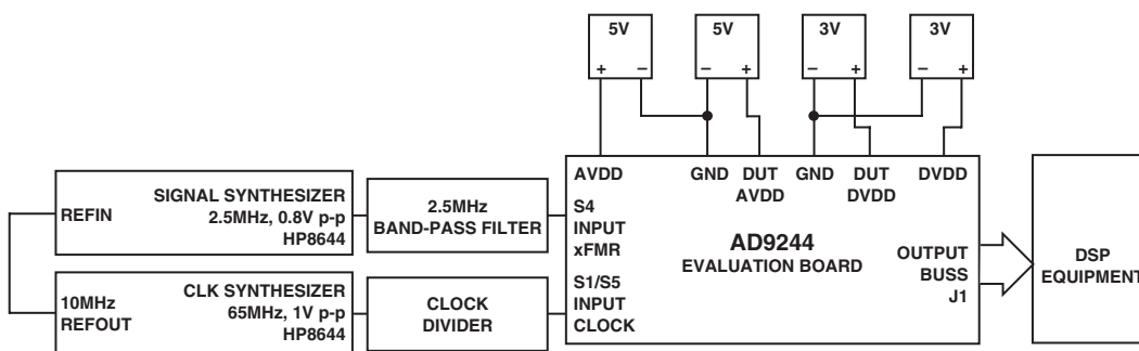
Figure 20. Evaluation Board Connections
