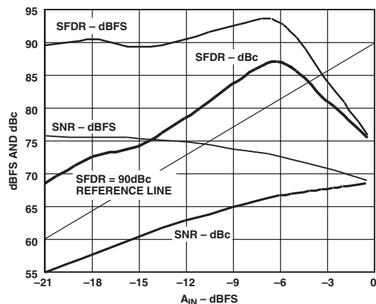
TPC 29. Driving ADC Inputs with Transformer and Balun SNR/SFDR vs. A_{IN} , f_{IN} = 240 MHz
