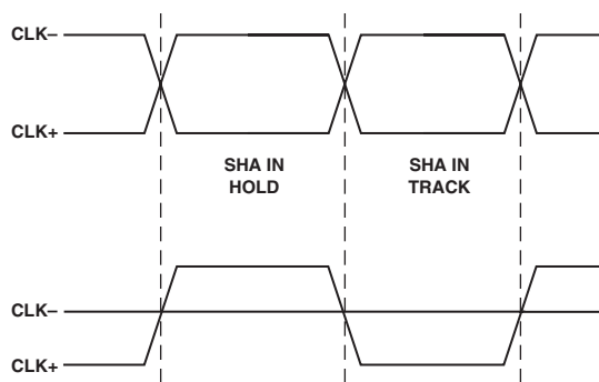
Figure 14. SHA Timing
