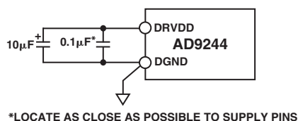
Figure 18. Digital Supply Decoupling
