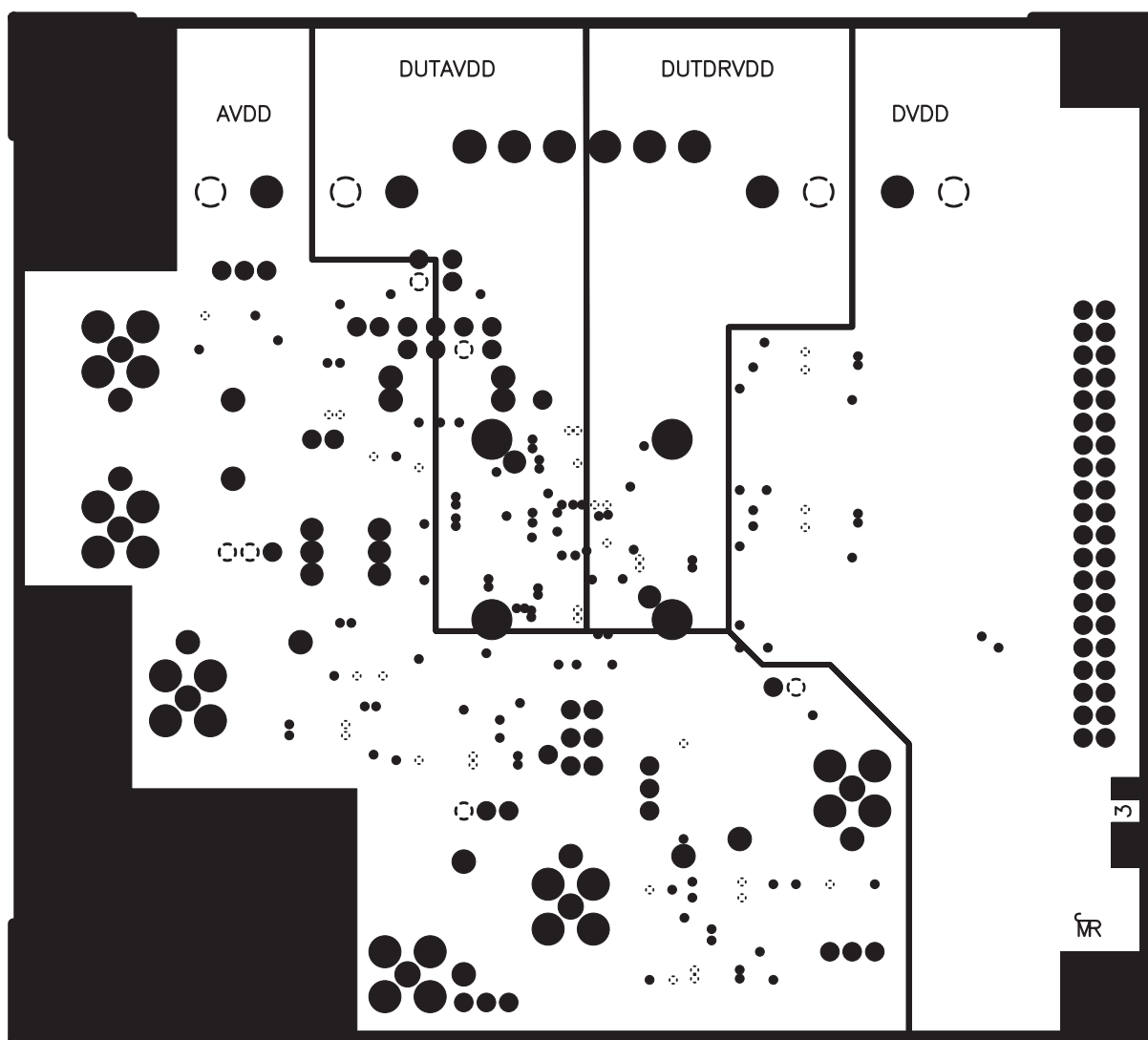
Figure 28. AD9244 Evaluation Board, PCB Layer 3 (Power Plane)
