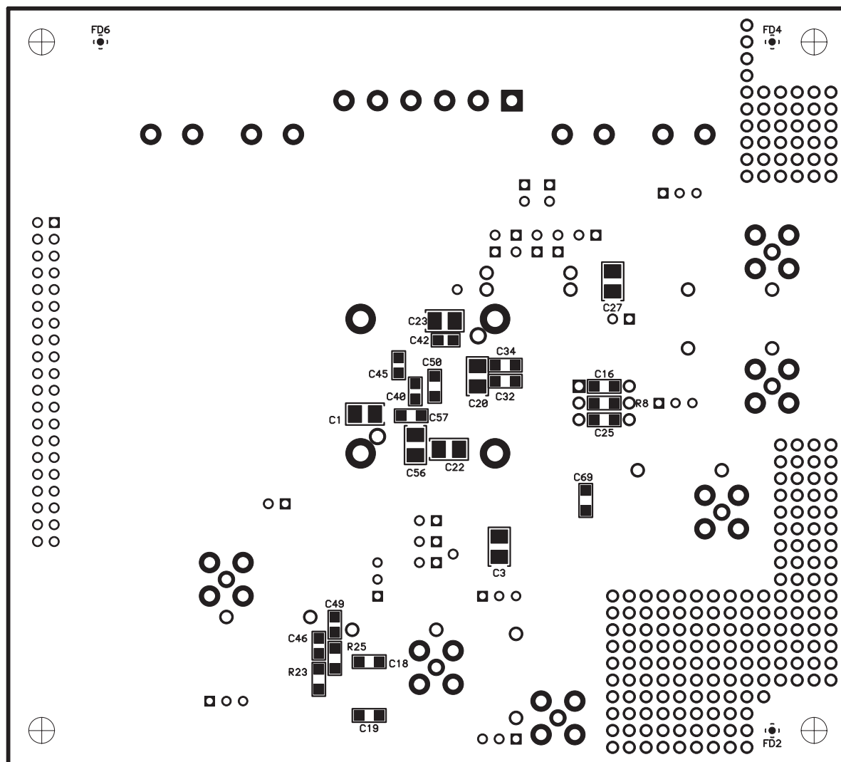
Figure 25. AD9244 Evaluation Board, PCB Assembly, Bottom
