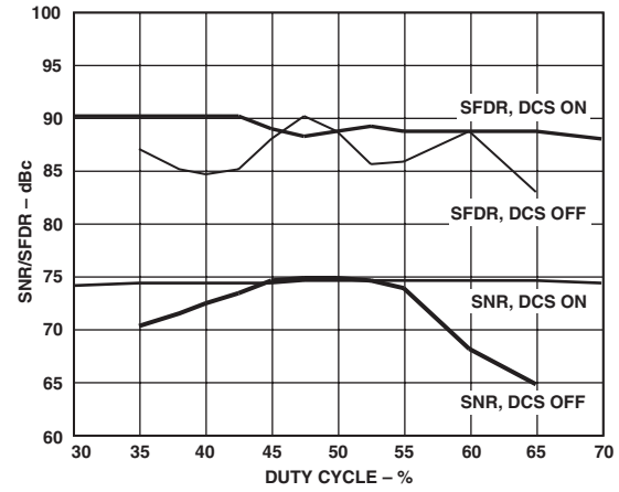
TPC 16. SNR/SFDR vs. Duty Cycle, f_{IN} = 2.5 MHz
