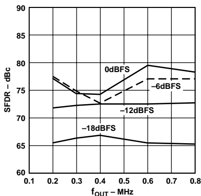
Figure 14. "Inband" SFDR vs. f_{OUT} @ 2 MSPS (DC to CLKIN/2 )
