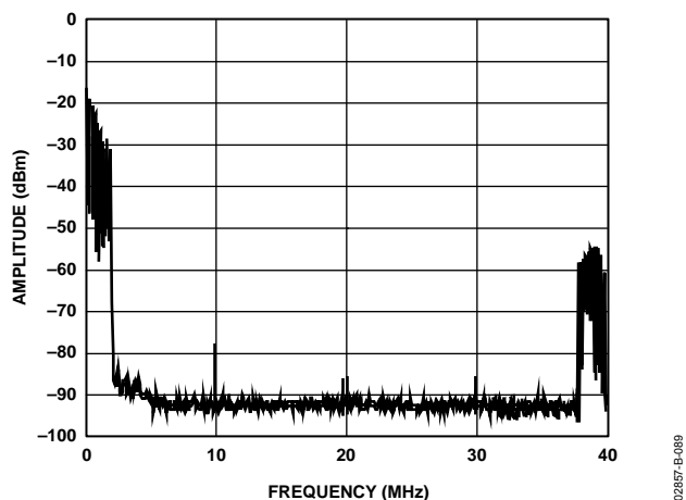
Figure 89. AD9773 Real DAC Output of Complex Input Signal Near Baseband (Positive Frequencies Only), Interpolation = 4x, No Modulation in AD9773
