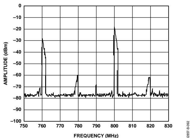
Figure 92. AD9773 Complex Output from Figure 91, Now Quadrature Modulated by AD8345 (LO = 800 MHz)
