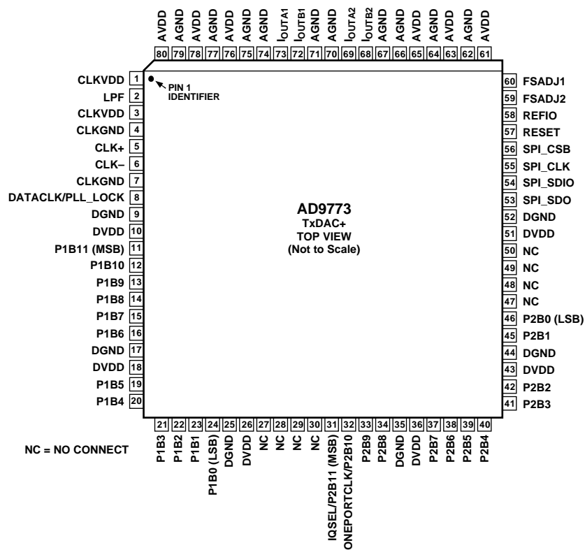
Figure 5. Pin Configuration
