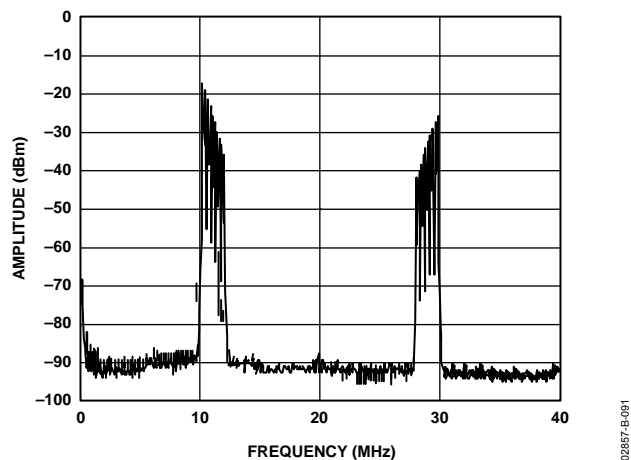
Figure 91. AD9773 Real DAC Output of Complex Input Signal Near Baseband (Positive Frequencies Only), Interpolation = 4x, Complex Modulation in AD9773 = +f_{DAC}/4
