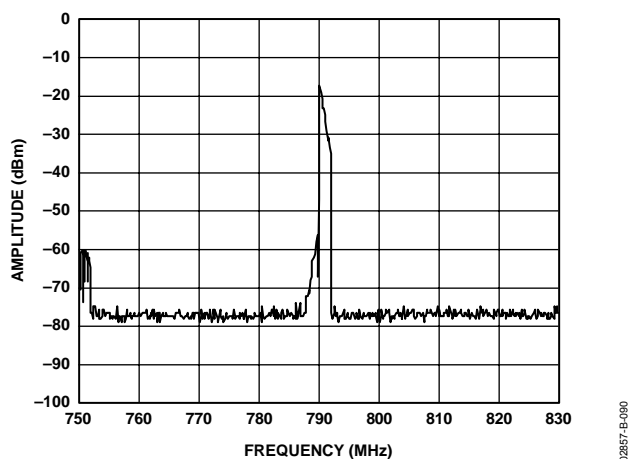
Figure 90. AD9773 Complex Output from Figure 89, Now Quadrature Modulated by AD8345 (LO = 800 MHz)
