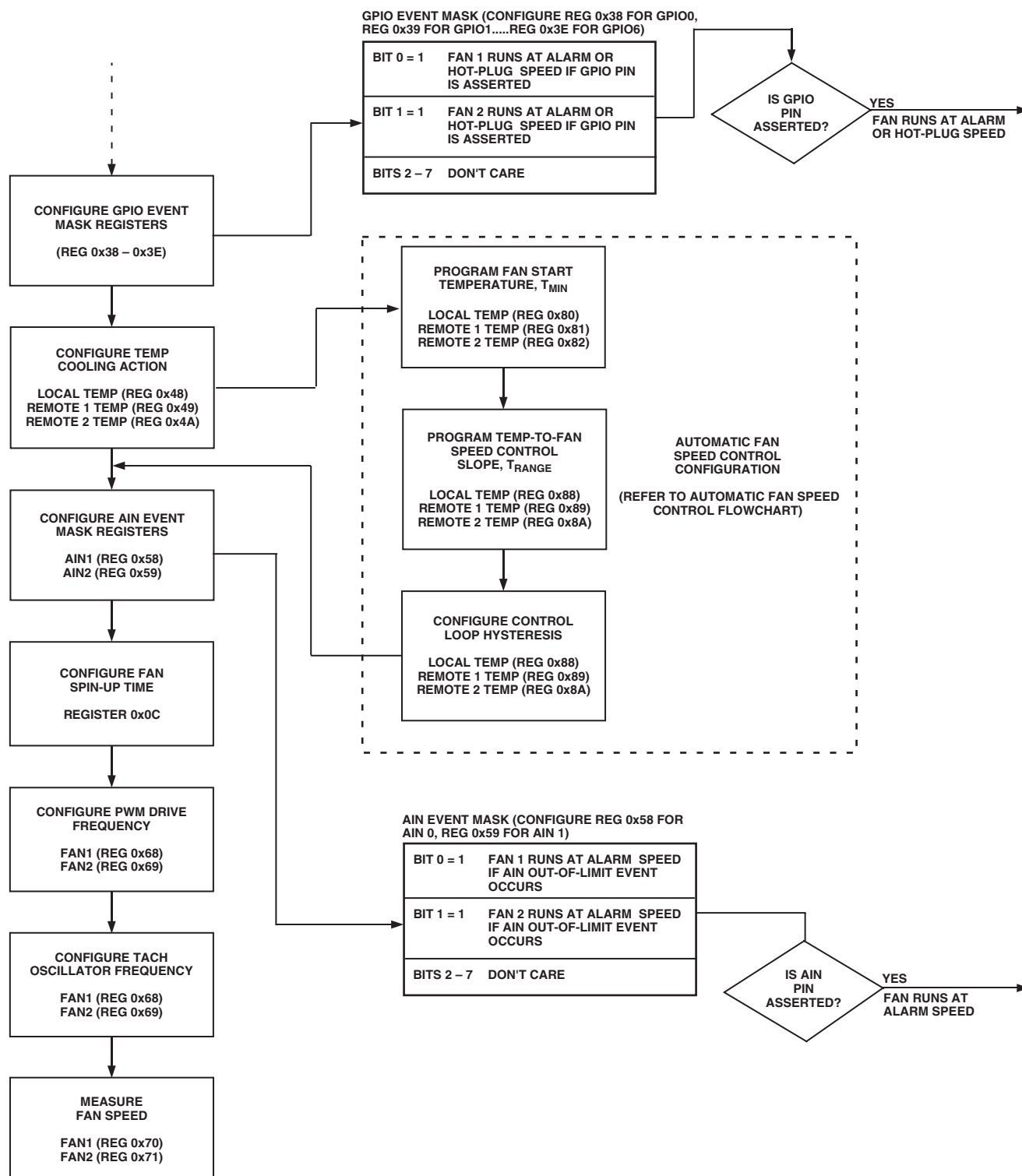
Figure 17. Fan Configuration Flowchart (Continued)
