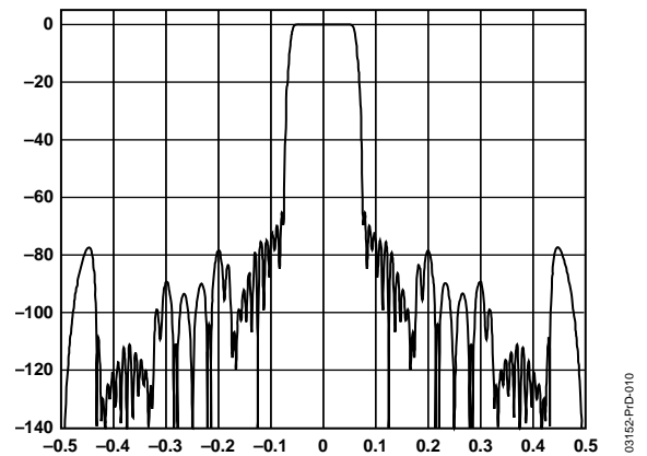
Figure 43. x8 Interpolation Filter Response
