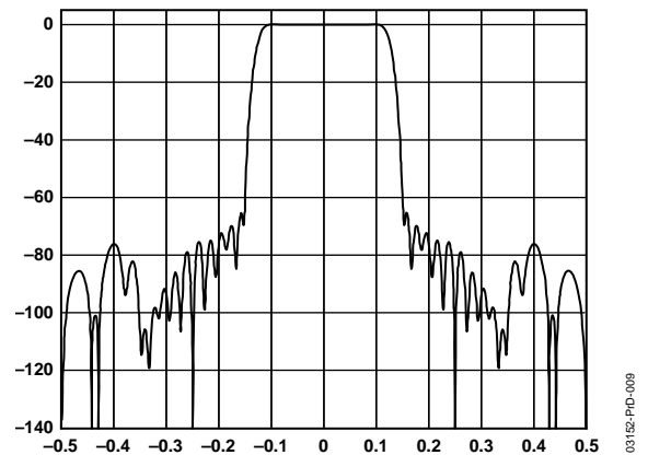
Figure 42. x4 Interpolation Filter Response
