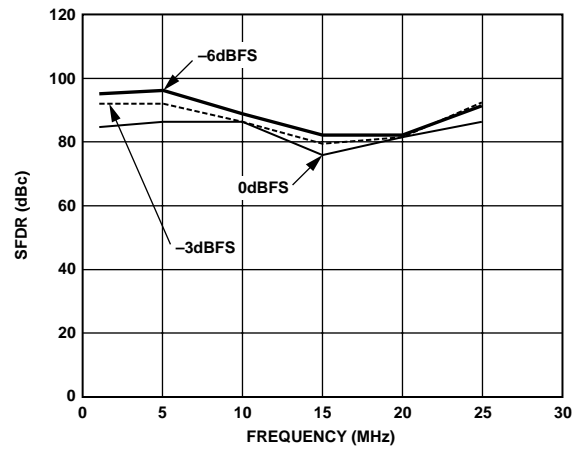
Figure 8. SFDR vs. Frequency, F_{DATA} = 62.5 MSPS, 8 \times Interpolation
