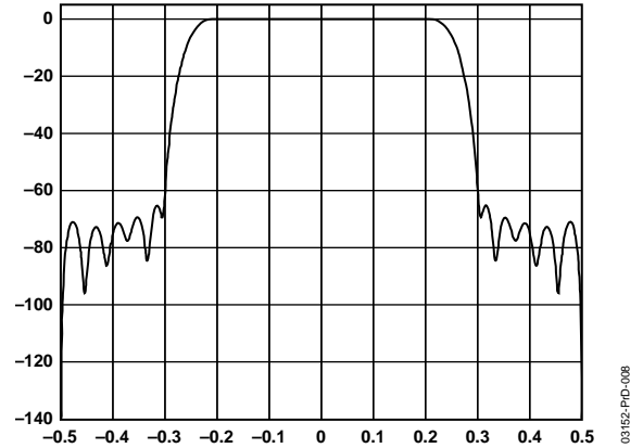
Figure 41. x2 Interpolation Filter Response
