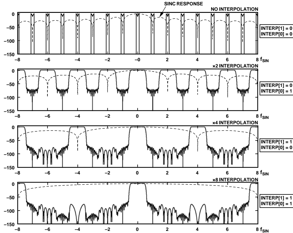
Figure 57. Interpolation Modes
