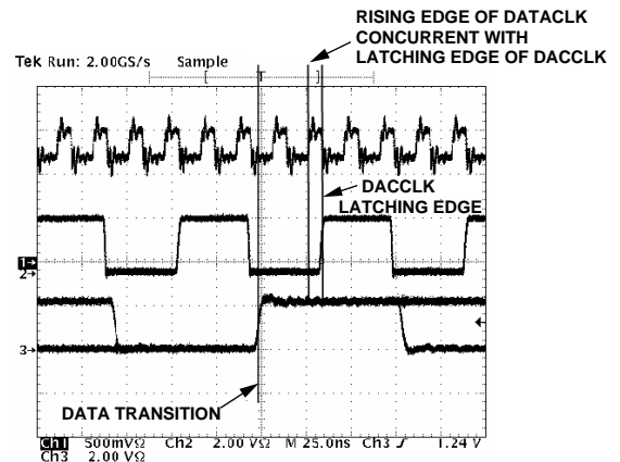
Figure 56. DATAADJ = 0001
