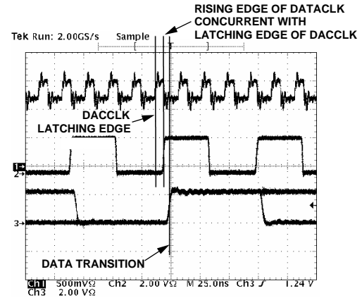
Figure 55. DATAADJ = 1111
